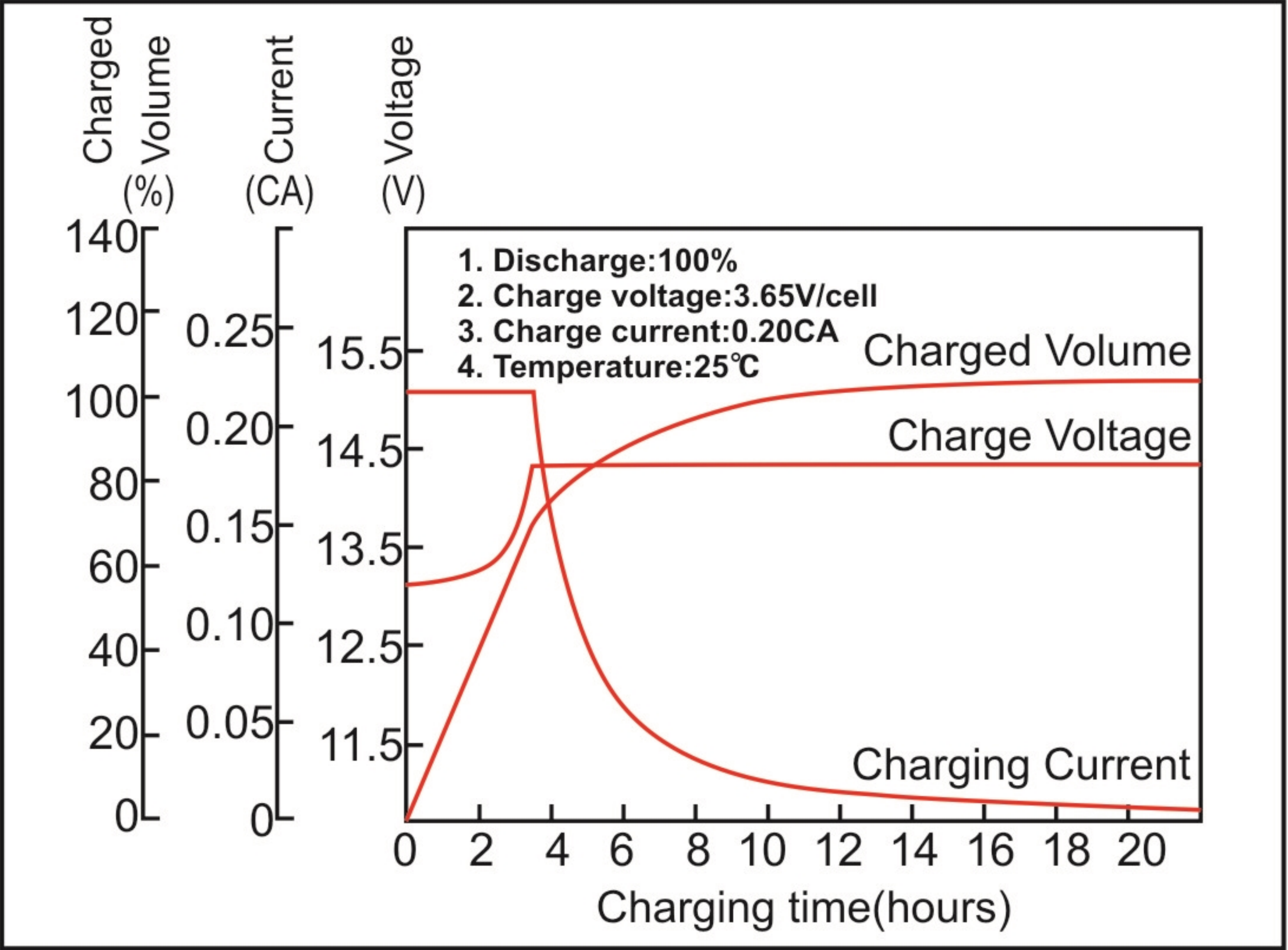
Constant voltage charging characteristics
