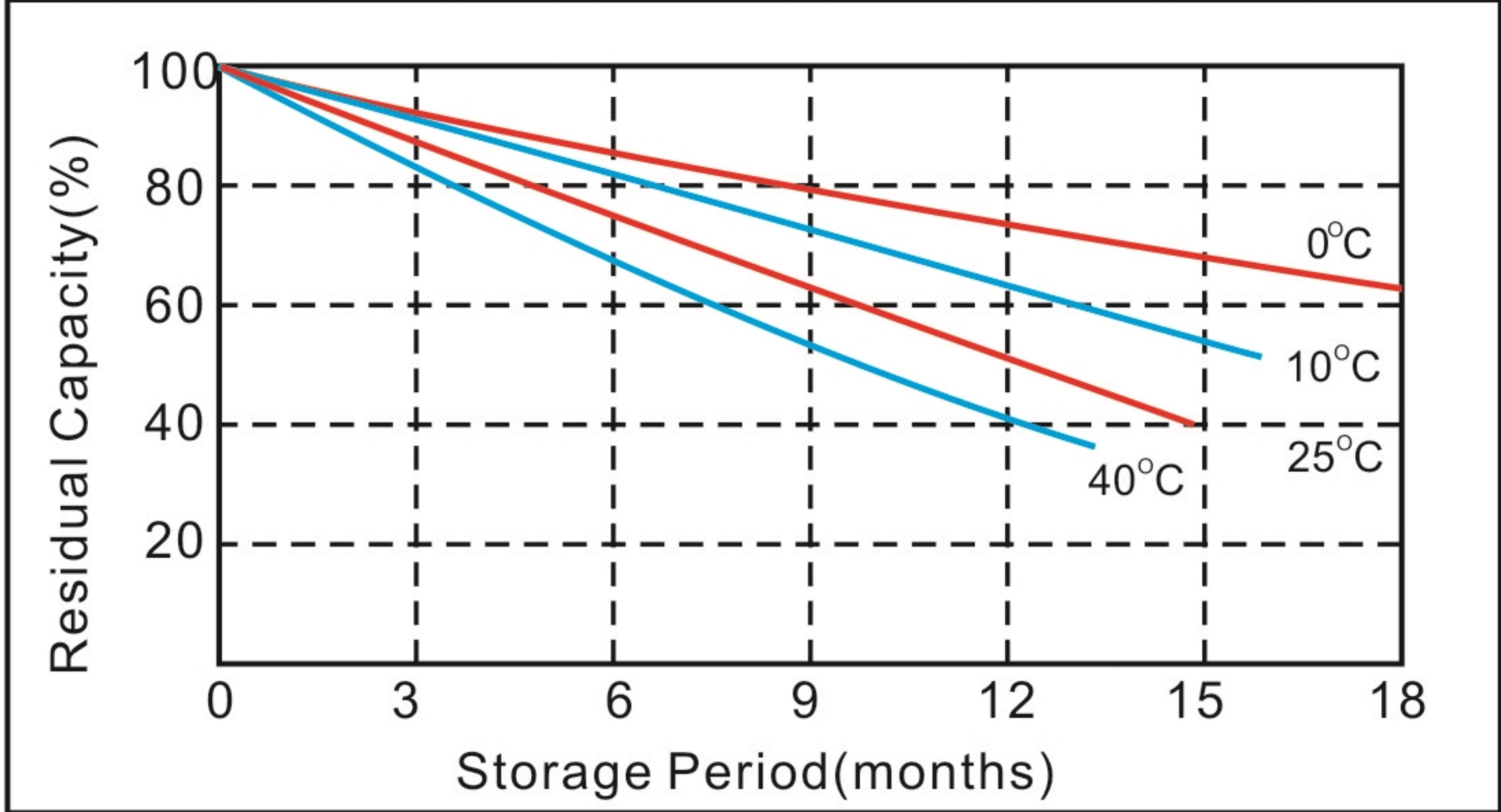
Constant Current Discharge Characteristics (A, 25°C)
